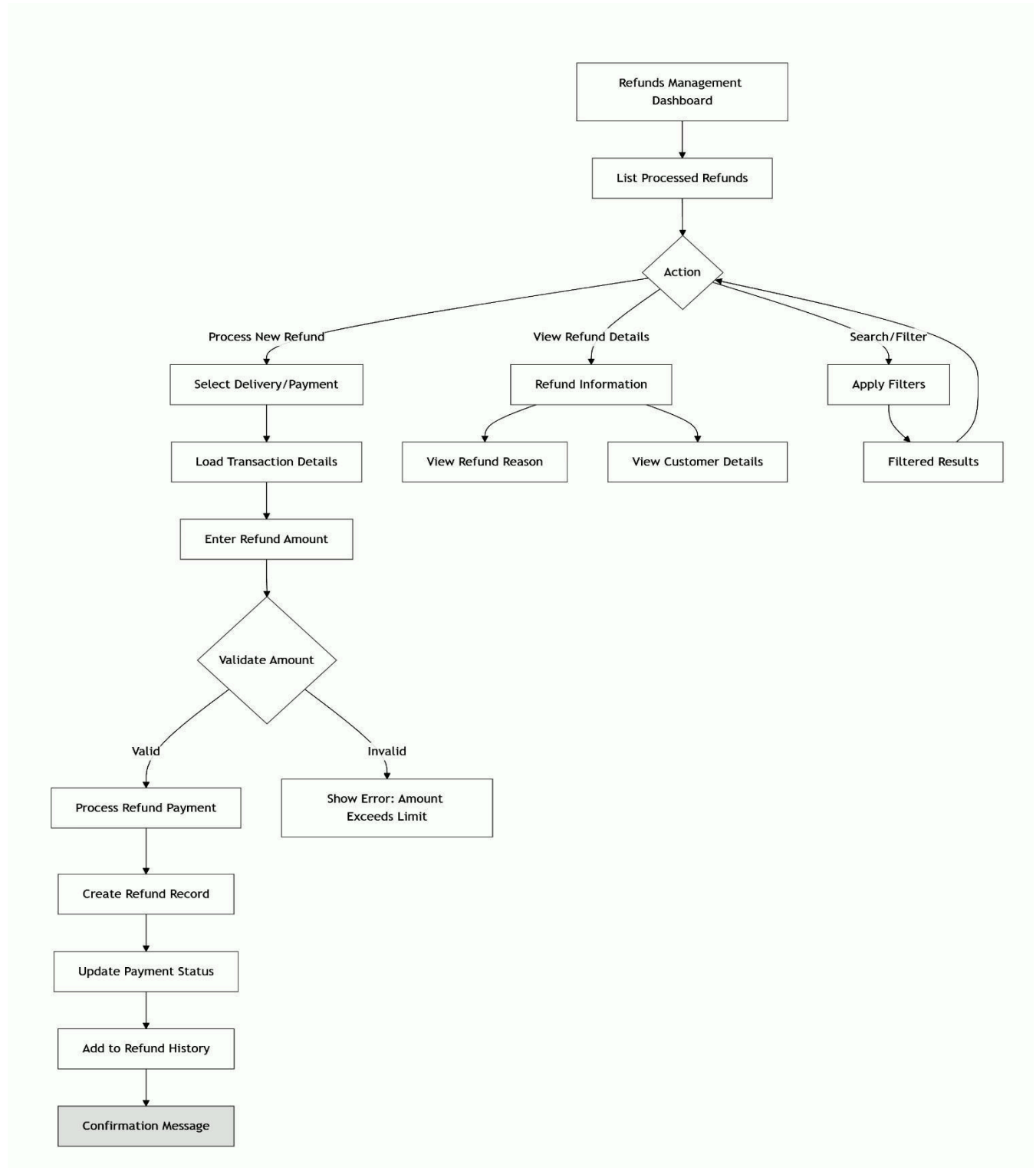
Figure 10.3: Administrator: Refund Management This Diagram shows how the administrator manages refunds.
